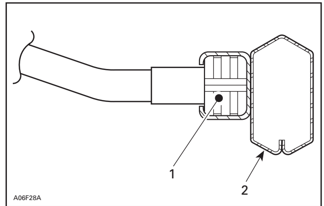
1. Sliding block 2. Swing arm
