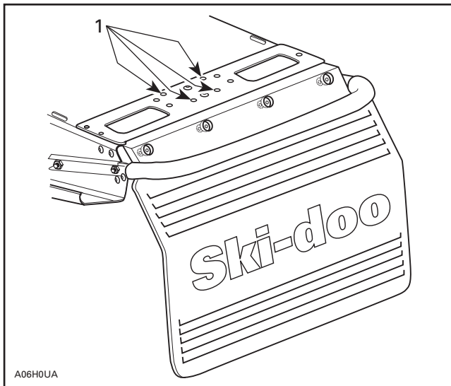
1. Pre-drilled holes
