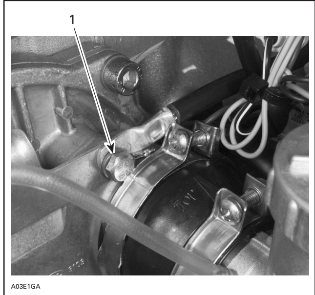
1. Connect BLACK ground cable here
